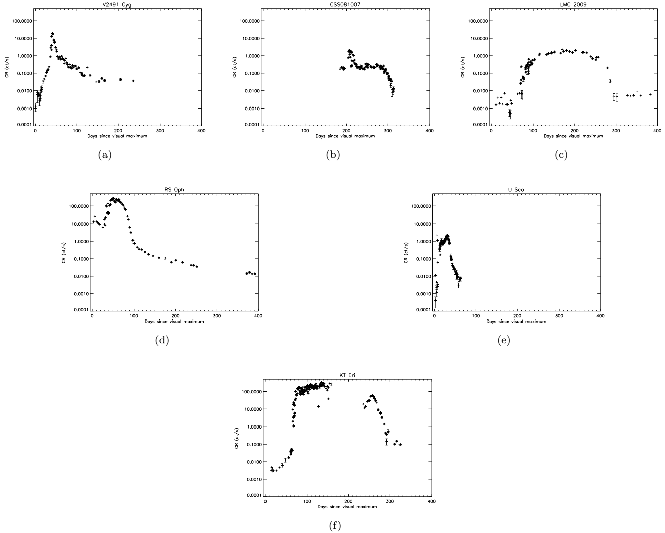
Figure 2. Inverted pyramid figure of six individual files. The nova are (a) V2491 Cyg, (b) HV Cet, (c) LMC 2009, (d) RS Oph, (e) U Sco, and (f) KT Eri. These individual figures are taken from Schwarz et al. (2011).
